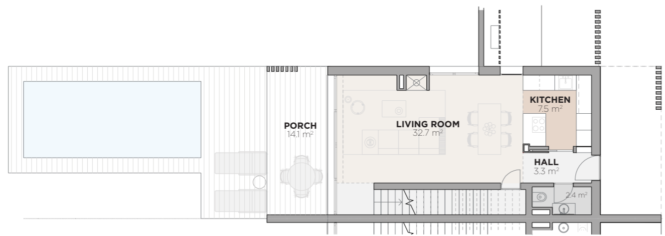
FLOOR 0
